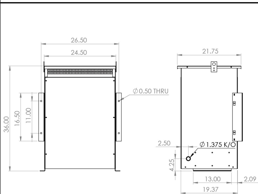
OUTLINE DRAWING
