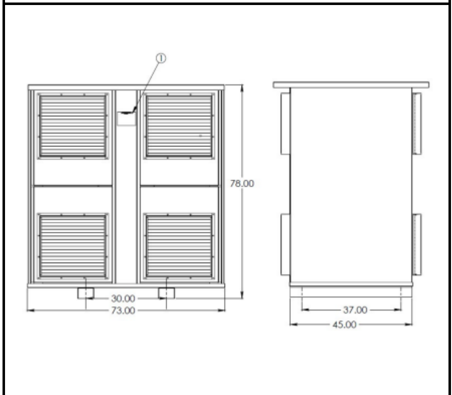
OUTLINE DRAWING
