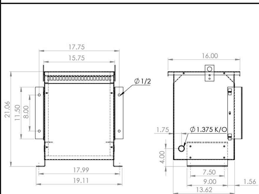
OUTLINE DRAWING
