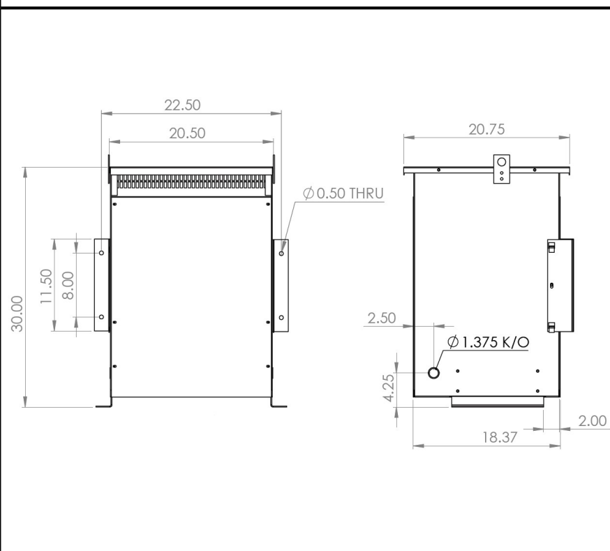
OUTLINE DRAWING
