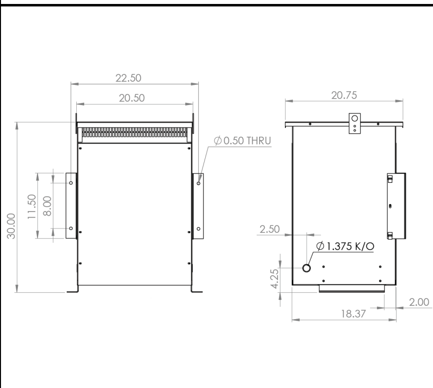
OUTLINE DRAWING
