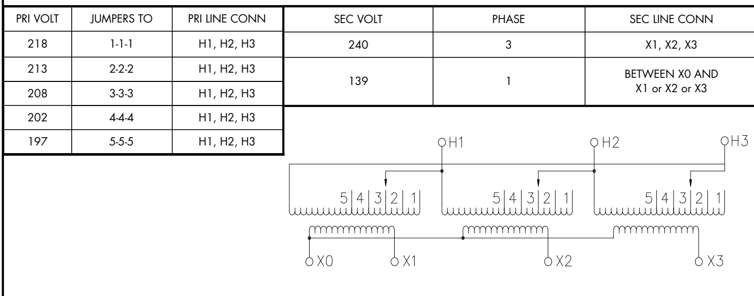
WIRING AND CONNECTION DIAGRAM
