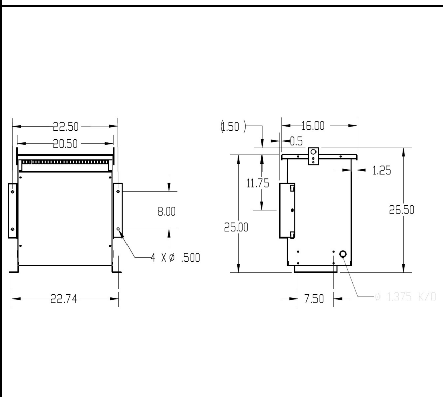
OUTLINE DRAWING
