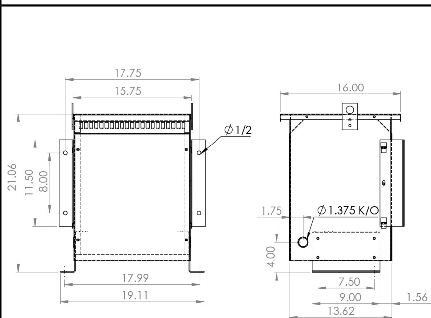
OUTLINE DRAWING
