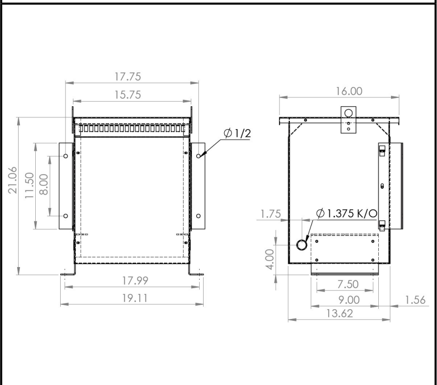
OUTLINE DRAWING
